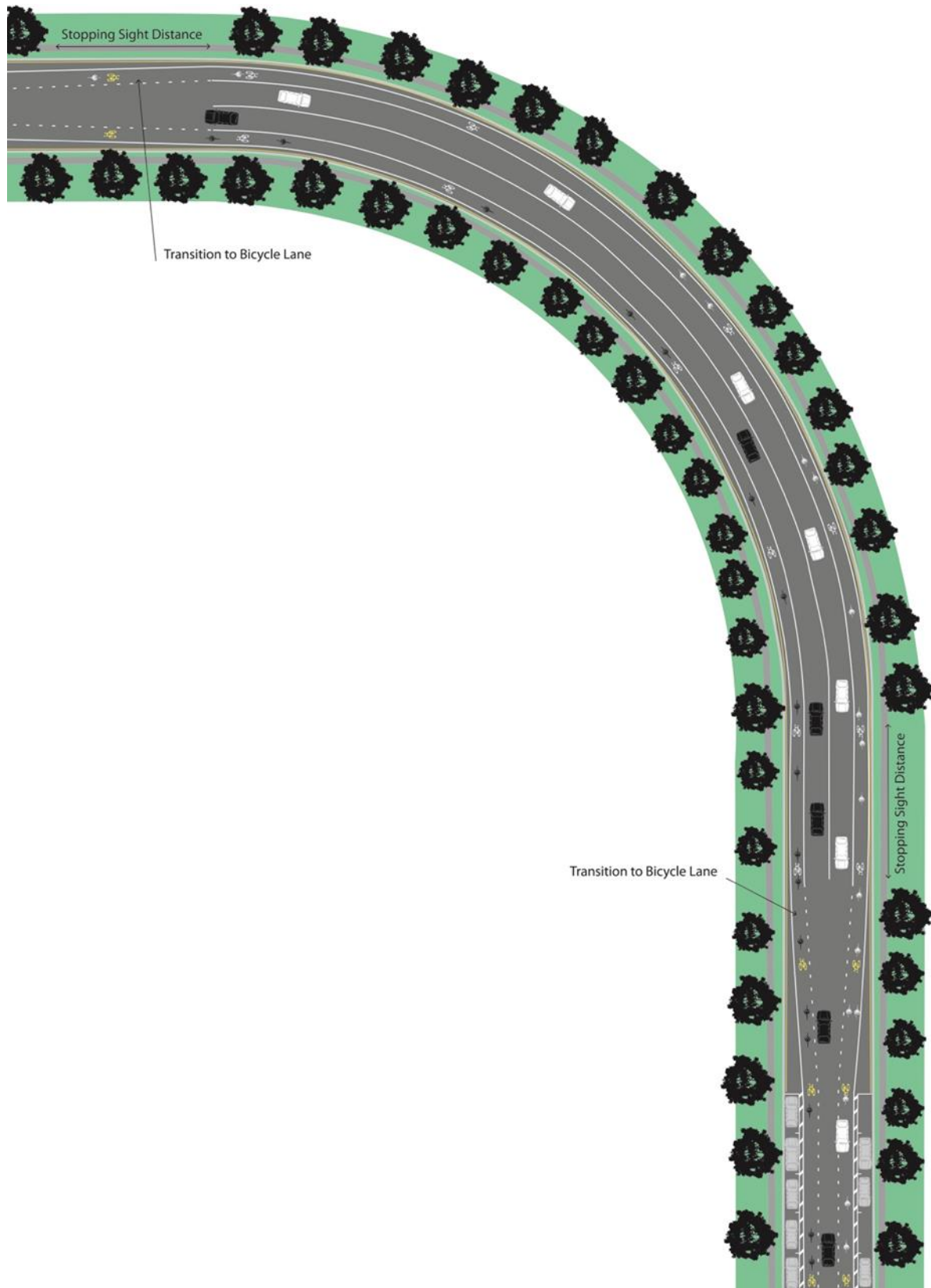
Figure A8 – Advisory Bicycle Lanes – Acceptable Curve treatment – Option 2 Transition to exclusive bicycle lanes with road centre line (requires removal of car parking)
